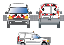
KIT R-B CL. A AVT+ARR+LAT - RENAULT KANGOO 2 PORTES (1997-2003)
