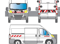
KIT R-B CL. B AVT+ARR+LAT - CITROËN JUMPER H2 (2006-2013)
